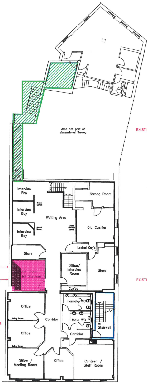
Proposed First Floor 1:100
